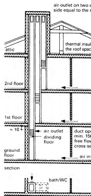
⑦ Single duct convection ventilation system
